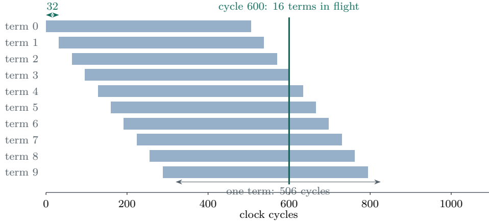
Figure 4: The modulo schedule (first ten of 128 terms). A term lasts 506 cycles and a new one starts every 32, so about 16 terms share the arithmetic units at any time.
