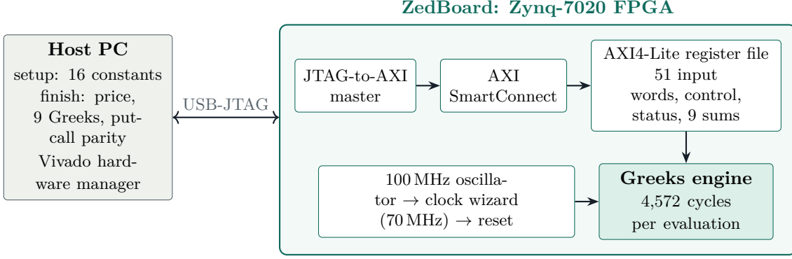
Figure 2: The system built on the ZedBoard (Vivado block design). The engine is driven over the JTAG cable, so the test exercises the datapath alone, with no processor software in the loop.
