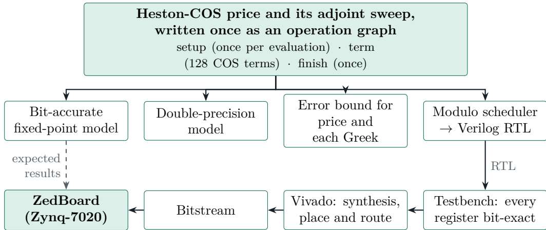
Figure 1: Design flow. The generator derives four artifacts from one operation graph; the RTL is checked register by register against the fixed-point model, implemented in Vivado and run on the ZedBoard, whose results are compared bit for bit with the same model.
