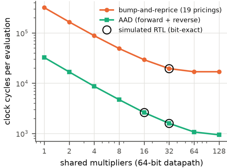
Figure 6: Cycles against shared multipliers (64-bit). Circled points were simulated as RTL and matched the schedule exactly.
