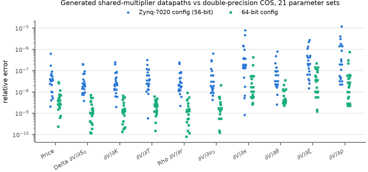
Figure 7: Relative error of every output for both designs over the 21 parameter sets.
