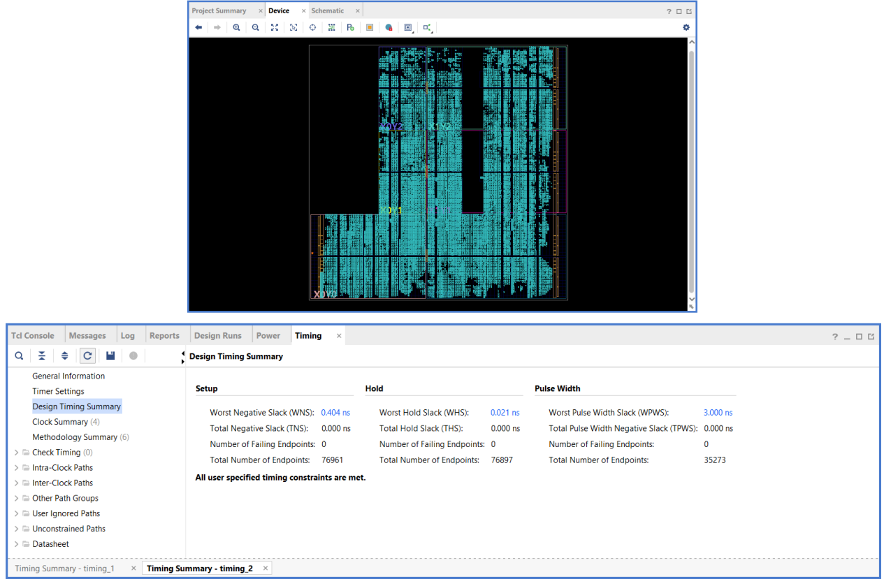
Figure 9: The placed design on the Zynq-7020 (top) and the timing summary of the ZedBoard build of 29 September: all constraints met at 70 MHz, 0 failing endpoints of 76,961 (bottom). The rebuild of 6 October with put-call parity and the refitted ranges also meets 70 MHz: WNS +0.458 ns, 0 failing endpoints of 76,672, and 394 more LUTs.
