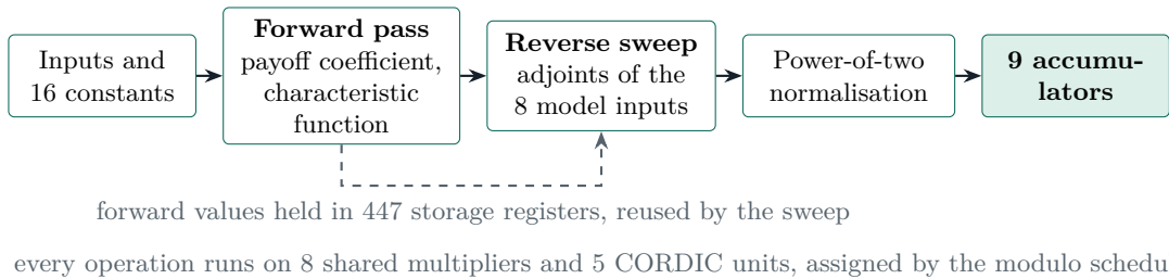
Figure 3: One COS term inside the engine. The adjoint sweep is part of the same datapath as the forward pass; there is no tape memory.
