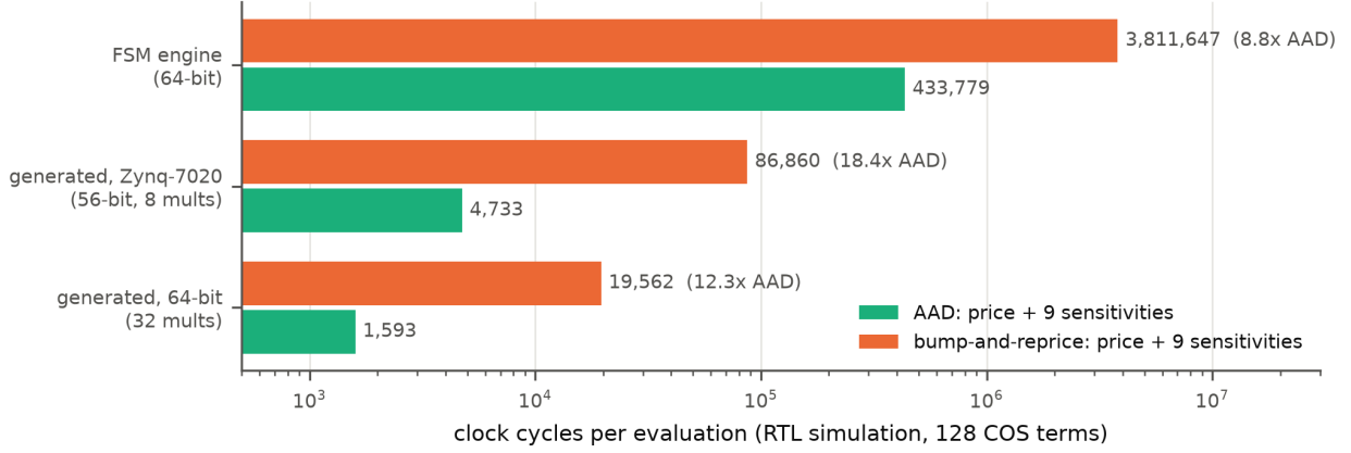
Figure 5: Cycles per evaluation, adjoint against bump-and-reprice on the same hardware (log scale).
